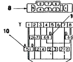
TP C SKYLIGHT WIPER SWITCH & DOME LIGHT
