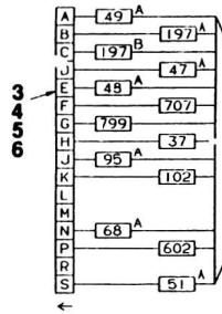
TP A FRONT CONSOLE CONNECTION
